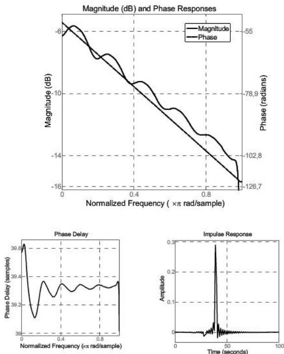
Fig.12. Simulation of the sample two-port network
