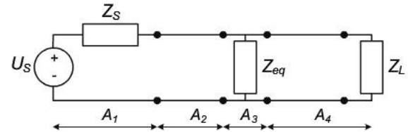
Fig. 10. Equivalent circuit for transmission line with one bridge tap connection
