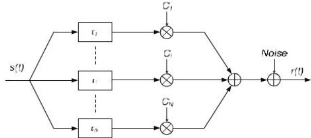
Fig.6. Multipath signal propagation representing power line channel
