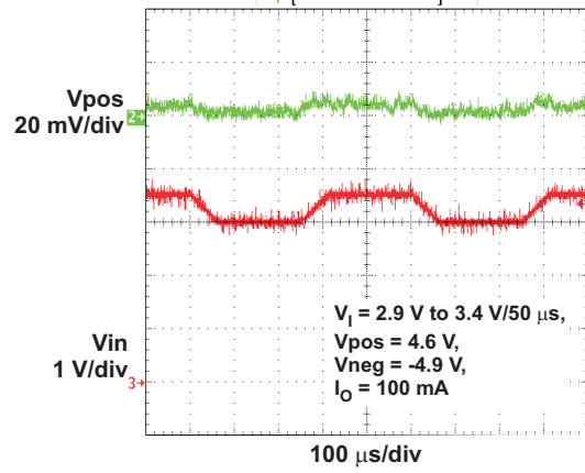
Figure 10. LINE TRANSIENT RESPONSE (100mA)
