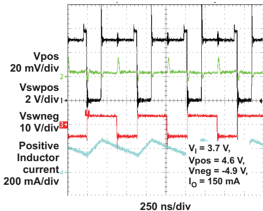
Figure 7. NOMINAL LOAD CURRENT OPERATION ( V_{IN} = 3.7\text{ V} )
