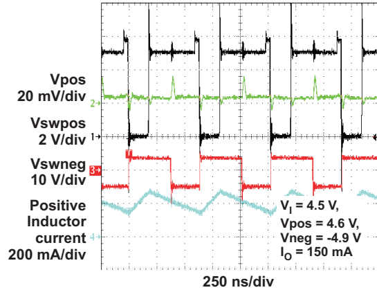
Figure 8. NOMINAL LOAD CURRENT OPERATION ( V_{IN} = 4.5\text{ V} )
