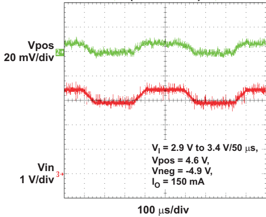
Figure 9. LINE TRANSIENT RESPONSE (150mA)
