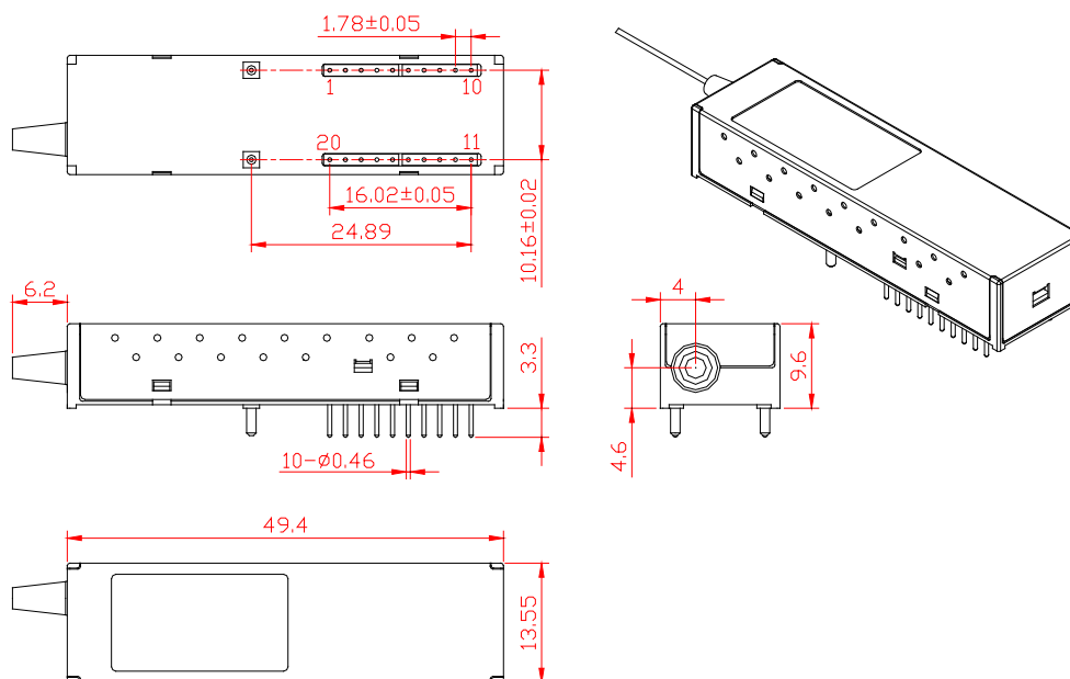
Figure5 Package outline
