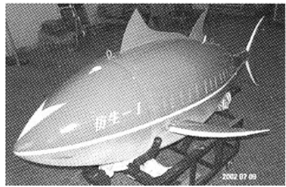
图 1 仿生水下机器人载体“仿生-I”号 Fig. 1 Bionic underwater vehicle “Fangsheng-I”
