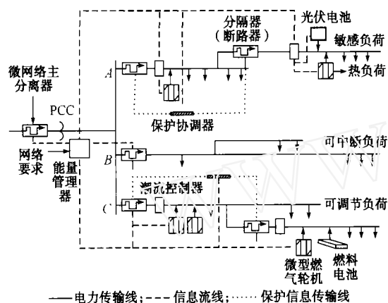
图1 CERTS提出的微电网结构 Fig.1 Topological structure of microgrid proposed by CERTS
