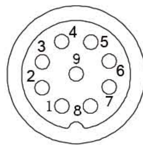
9pin
