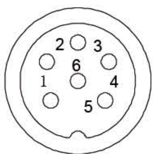
6pin
