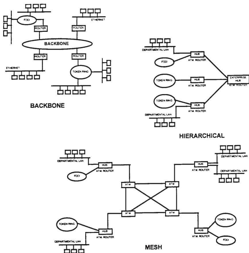
FIG. 2 Internetwork Topology
